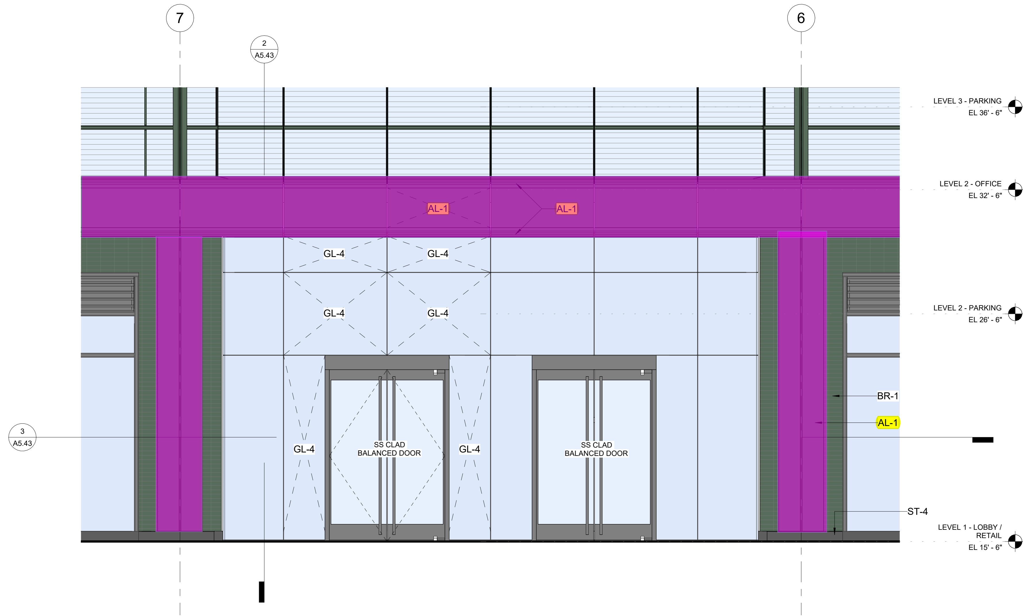
1 ELEVATION 3/8" = 1'-0"
