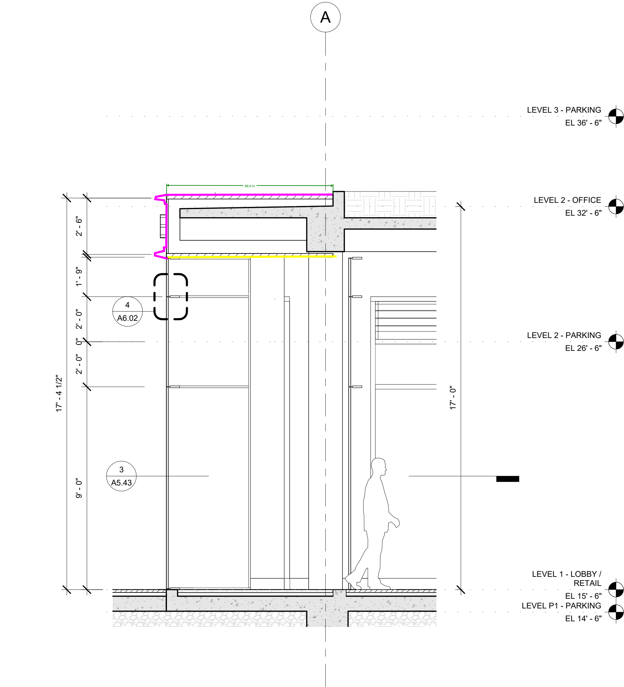
2 SECTION 3/8" = 1'-0"
