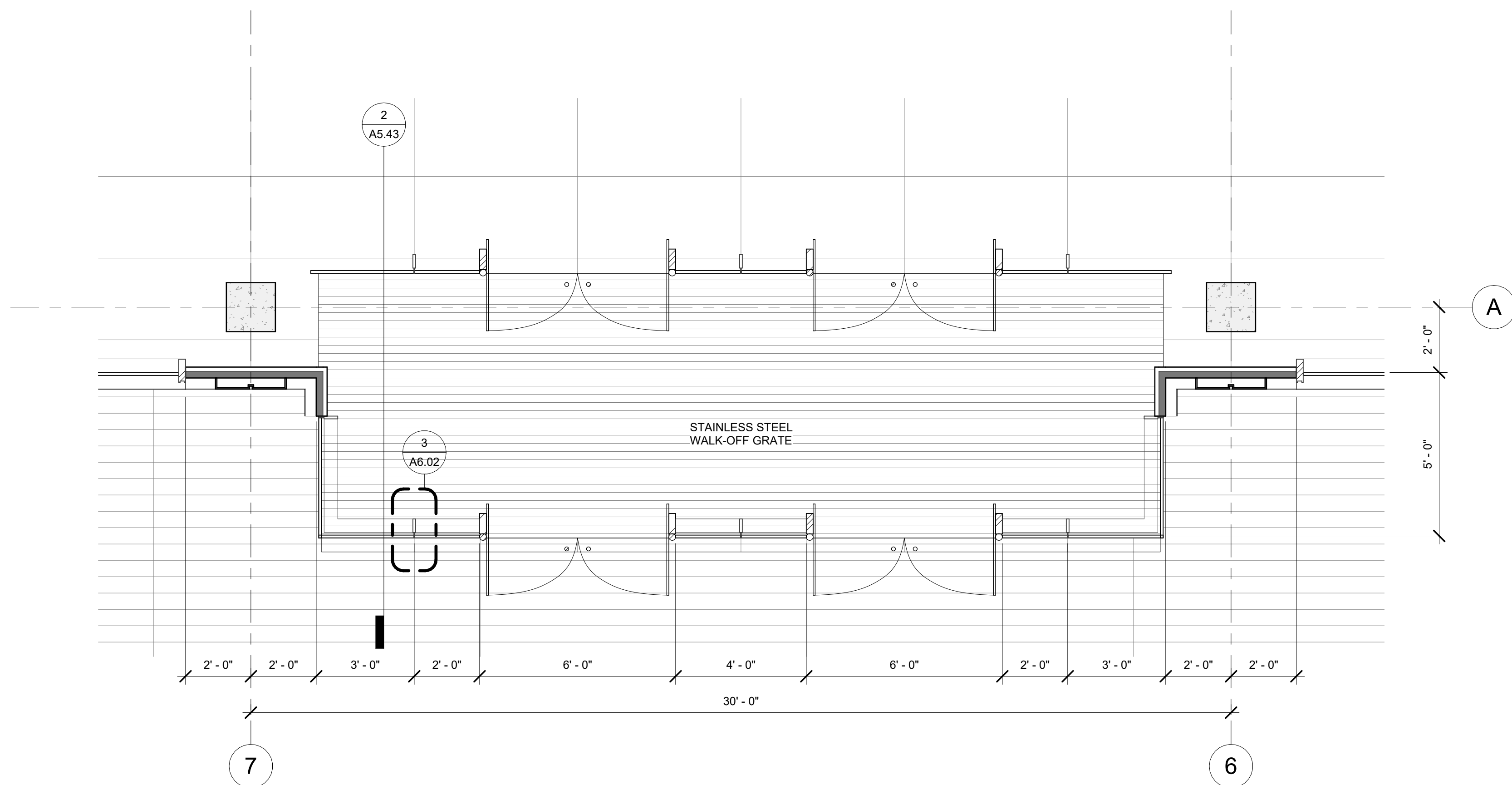
3 PLAN 3/8" = 1'-0"
